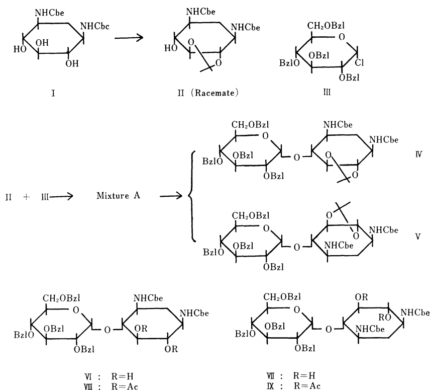
Chart 1. Cbe: \text{CO}_2\text{C}_2\text{H}_5 Bzl: \text{CH}_2\text{C}_6\text{H}_5
